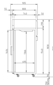
SIDE VIEW
